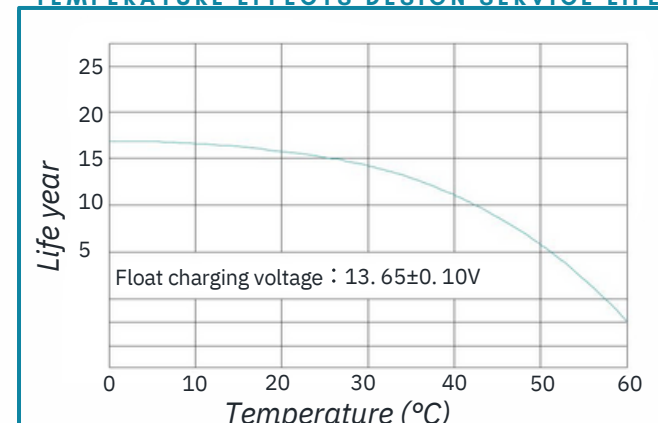
TEMPERATURE EFFECTS DESIGN SERVICE LIFE
