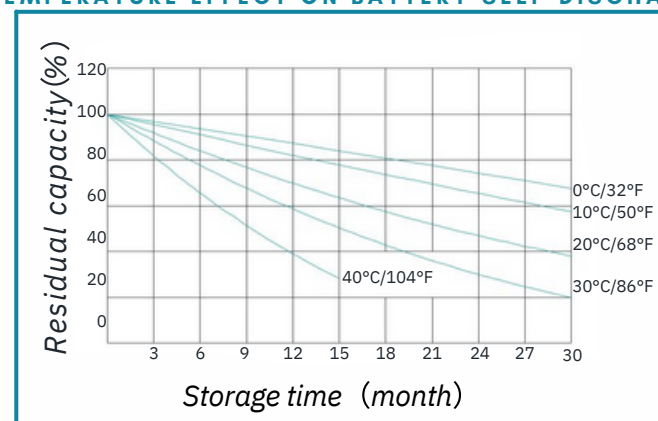
TEMPERATURE EFFECT ON BATTERY SELF-DISCHARGE
