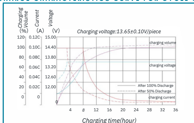
CHARGE CHARACTERISTICS CURVE FOR CYCLE USE
