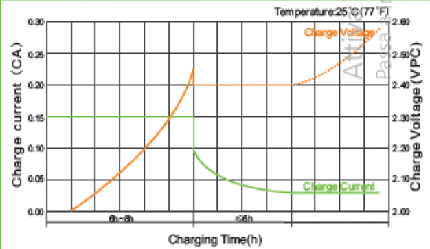
Charge Characteristic Curve For Cycle Use(IUIU)
